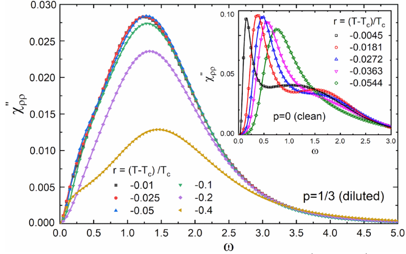
Figure 1. Scalar spectral function \chi''_{\rho\rho}(\vec{q}=0, \omega) . Main panel: dilution p=1/3 . Inset: clean case ( p=0 ). [1]
